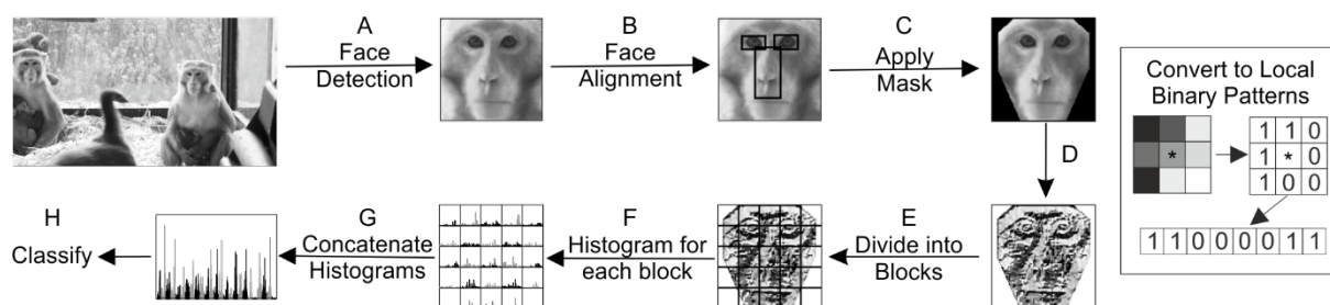
Figure 2. Diagram of face recognition stages. Inset, calculating the local binary pattern for a single pixel (*).
