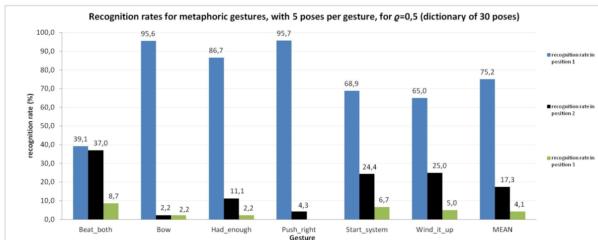
Fig. 5 Recognition rates for metaphoric gestures of MSRC-12 dataset.
