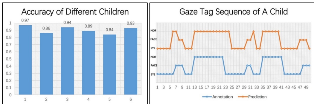
Figure 2. Accuracy of gaze classification on our dataset and predicted fixation tag sequence
