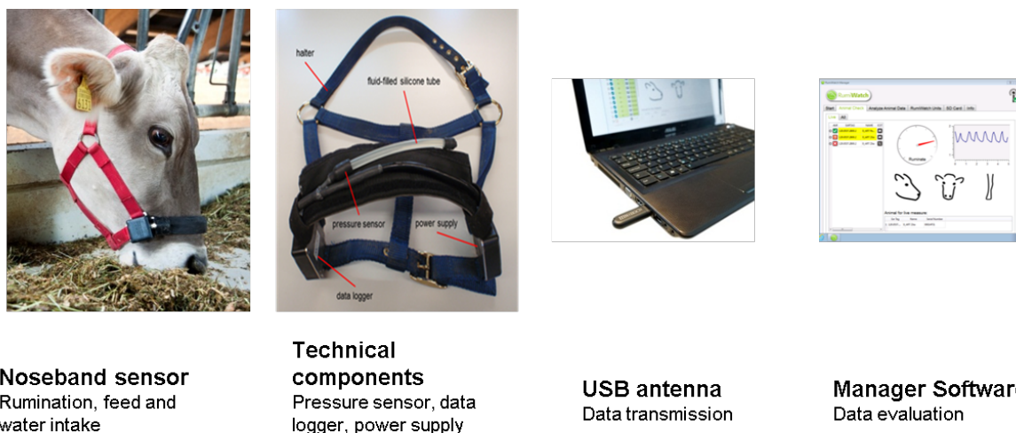
Fig. 1. The components of the RumiWatchSystem.
